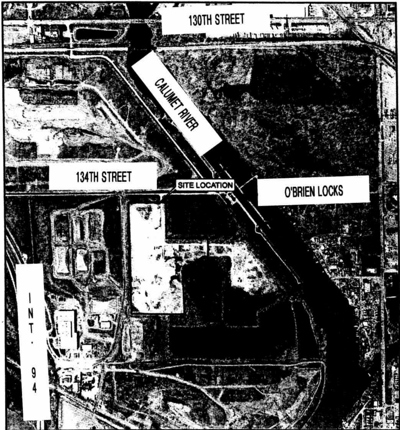
FIGURE 2-2 SITE LAYOUT MAP 2025 EAST 134TH STREET CHICAGO, COOK COUNTY, ILLINOIS
