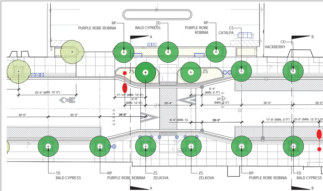
MID BLOCK CROSSING - LANDSCAPE PLAN
