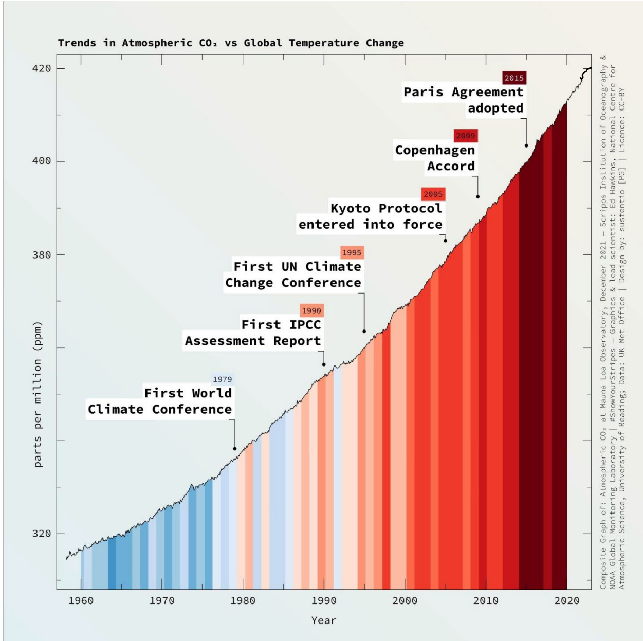
FIGURE 2: MONTHLY MEAN CARBON DIOXIDE AT MAUNA LOA OBSERVATORY, HAWAII
