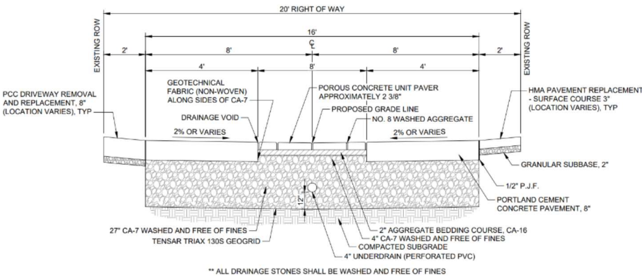
PROPOSED TYPICAL SECTION (ALL ALLEY LOCATIONS)
