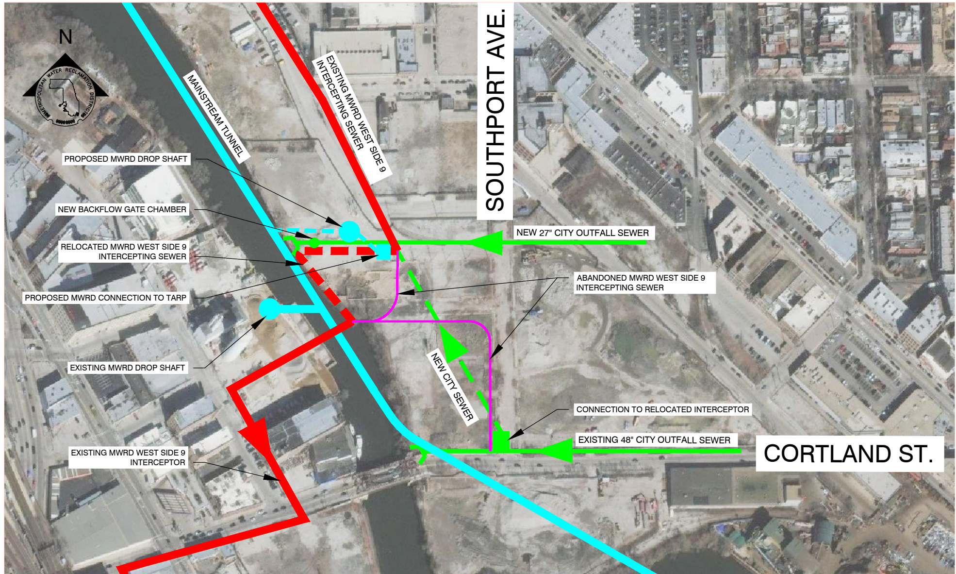
EXHIBIT 1 : PROPOSED MWRD LINCOLN YARDS INFRASTRUCTURE MODIFICATIONS AND DROP SHAFT
