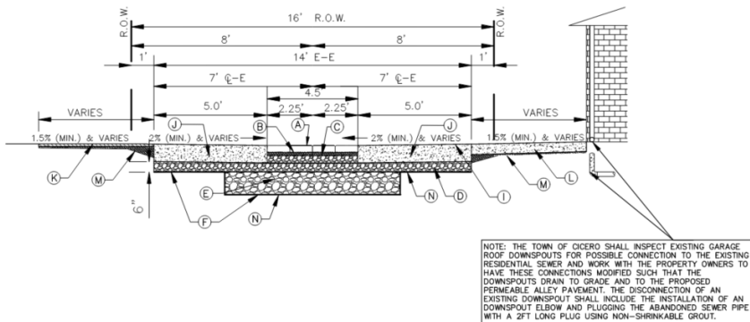
PROPOSED SECTION - NO STORM SEWER
