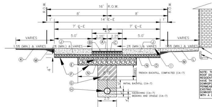
PROPOSED SECTION - WITH STORM SEWER
