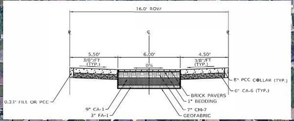
Typical Green Alley Section
