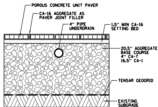
PERMEABLE PAVER DETAIL
